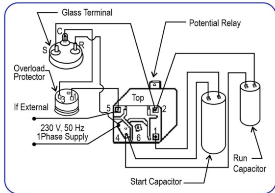
CAPACITOR START CAPACITOR RUN (CSCR)
