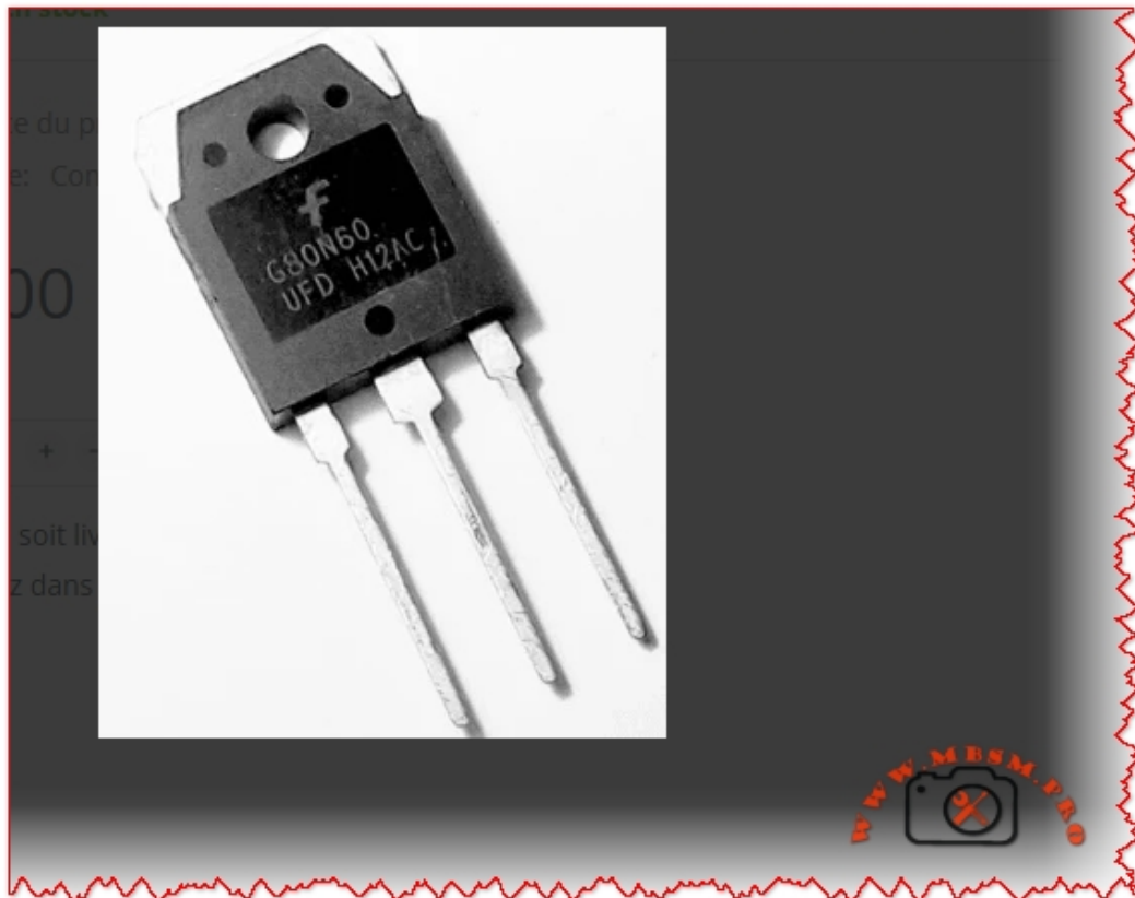
Transistor IGBT, G80N60UFD, 600 V, 80 A mbsmpro
